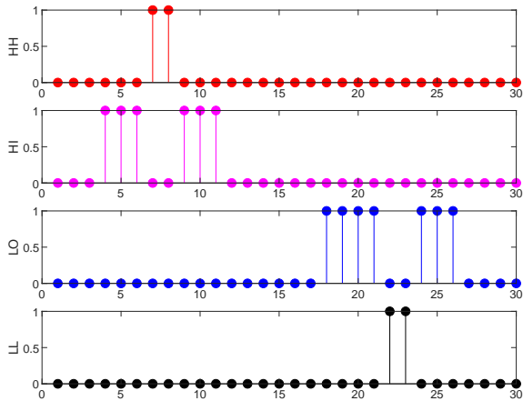
Fig. 1. Binary alarm sequences for four IA tags
